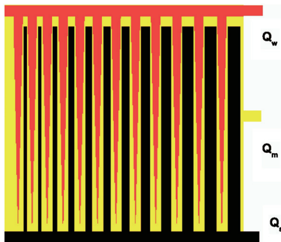
Figure 7. [Colour online] Three anodes are shown by different colours. They are separated by very narrow insulating gaps ( \sim 30 \mu\text{m} ). The area of black anodes (strip) linearly increases in width, as they progress from left to right ( x direction), the area of each of the red anodes (wedge) linearly increases in width, as they progress from the bottom to the top ( y direction), and the yellow anode (meander) zigzags between the black and red anodes.
