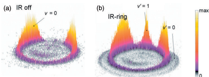
Figure 14. [Colour online] The 3D representation of the \text{CHD}_2 product raw image of the \text{Cl} + \text{CH}_2\text{D}_2 (v_6=0, 1) \rightarrow \text{HCl} + \text{CHD}_2 (v_i=0) reaction from the study of Riedel et al. [224]. (a) No excitation, v_6=0 . (b) \text{CH}_2\text{D}_2 molecules are excited into the v_6=1 state by radiation of an infrared laser when they pass through a multipass ring. The labels refer to the vibrational state of the HCl products. Reprinted from reference [110] with permission from AIP.
