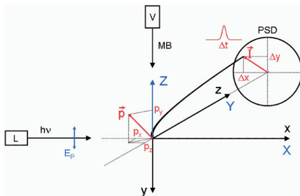
Figure 2. [Colour online] Laser based (XYZ, \text{blue}) and spectrometer based (xyz, \text{black}) coordinate systems. The PSD is situated on the z axis, the laser beam (L) and the molecular beam (MB) propagate in x and y directions, respectively. The curved trajectory along the z axis shows how the initial momentum vector \vec{p} is transformed into the measured image vector \vec{I} .
